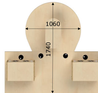
Conf. D - 2
